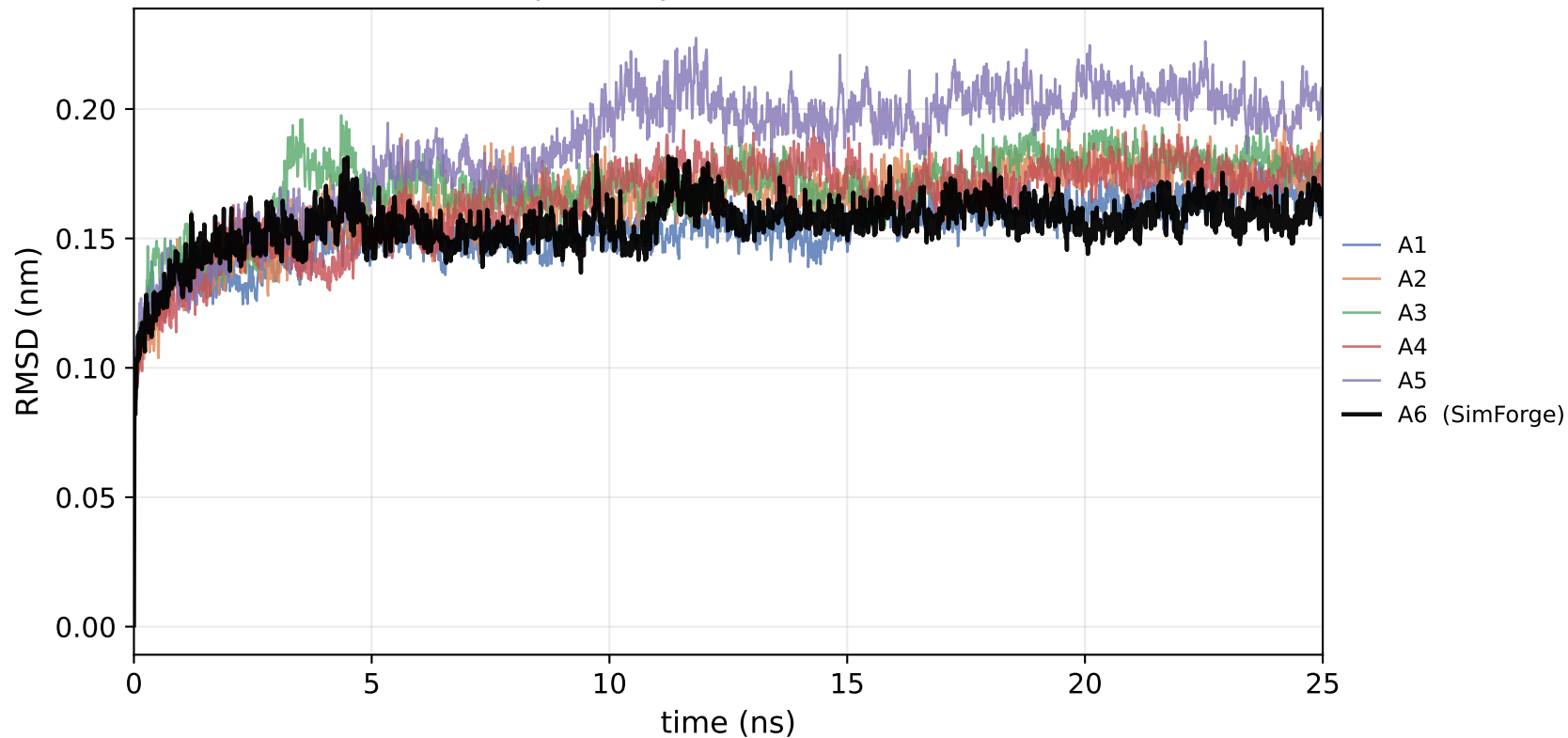
AA (alpha-amylase) - Protein RMSD
