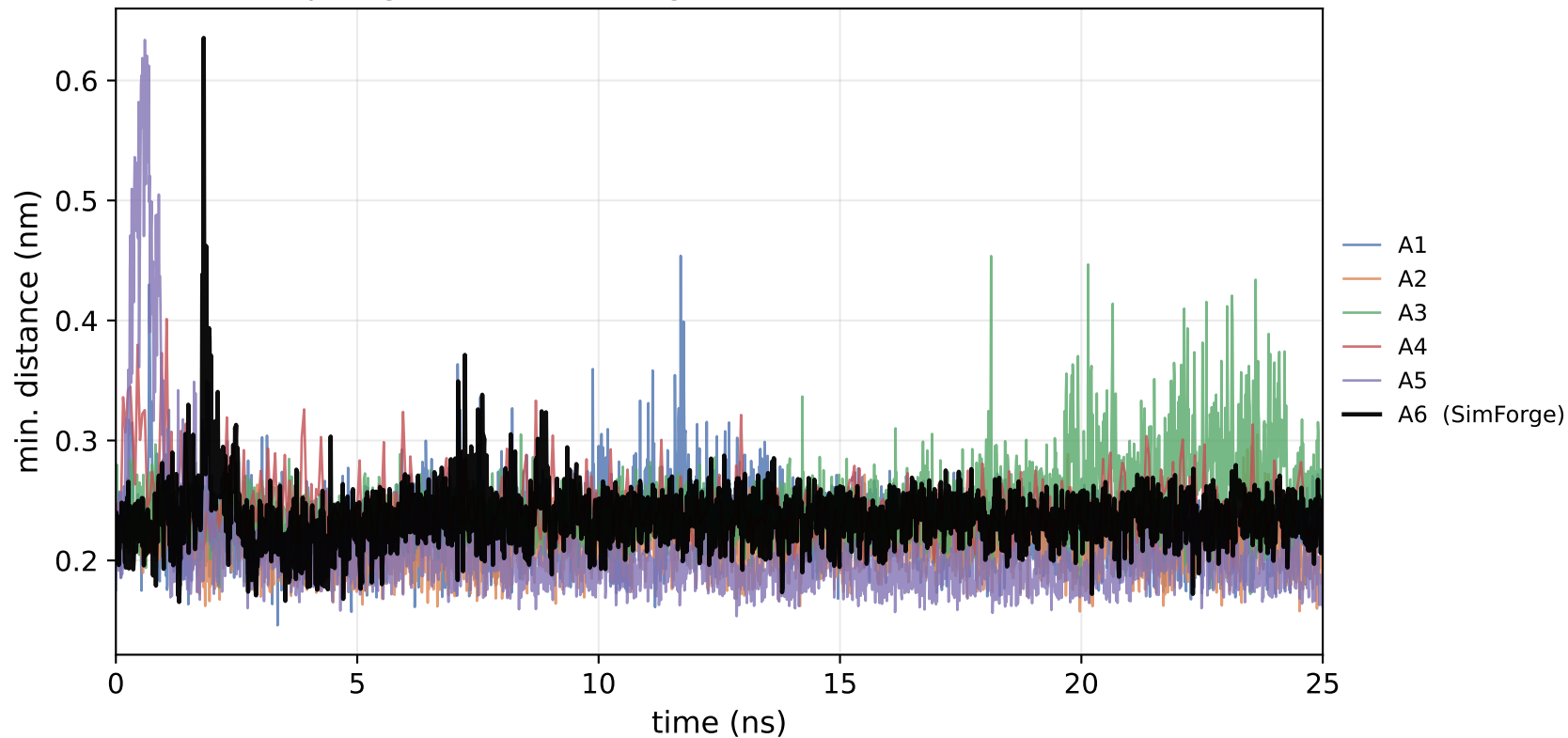
AG (alpha-glucosidase) - Ligand-active-site minimum distance
