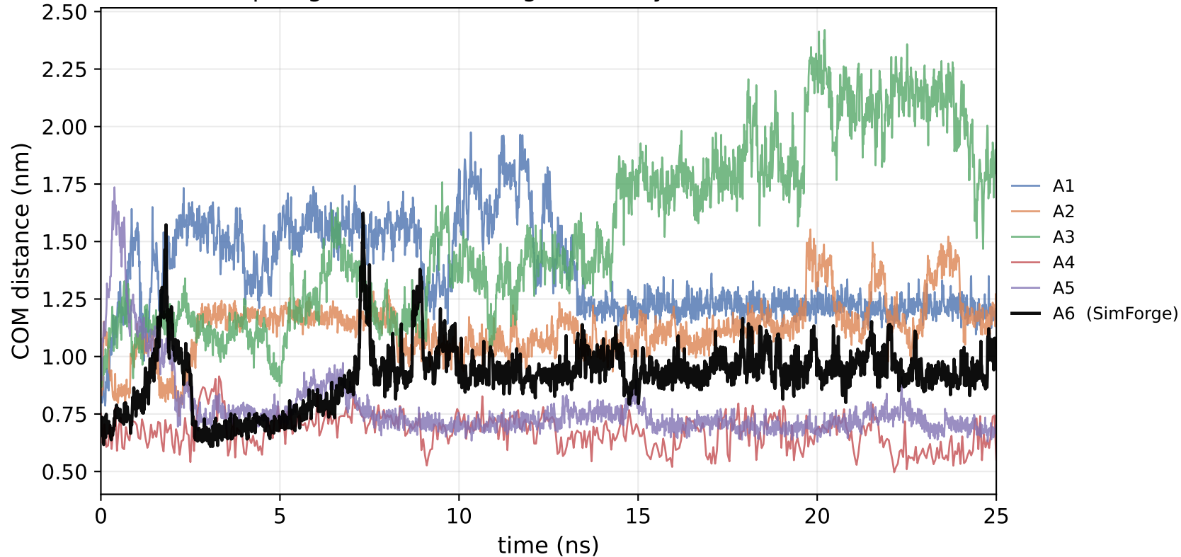
AG (alpha-glucosidase) - Ligand-catalytic-site COM distance
