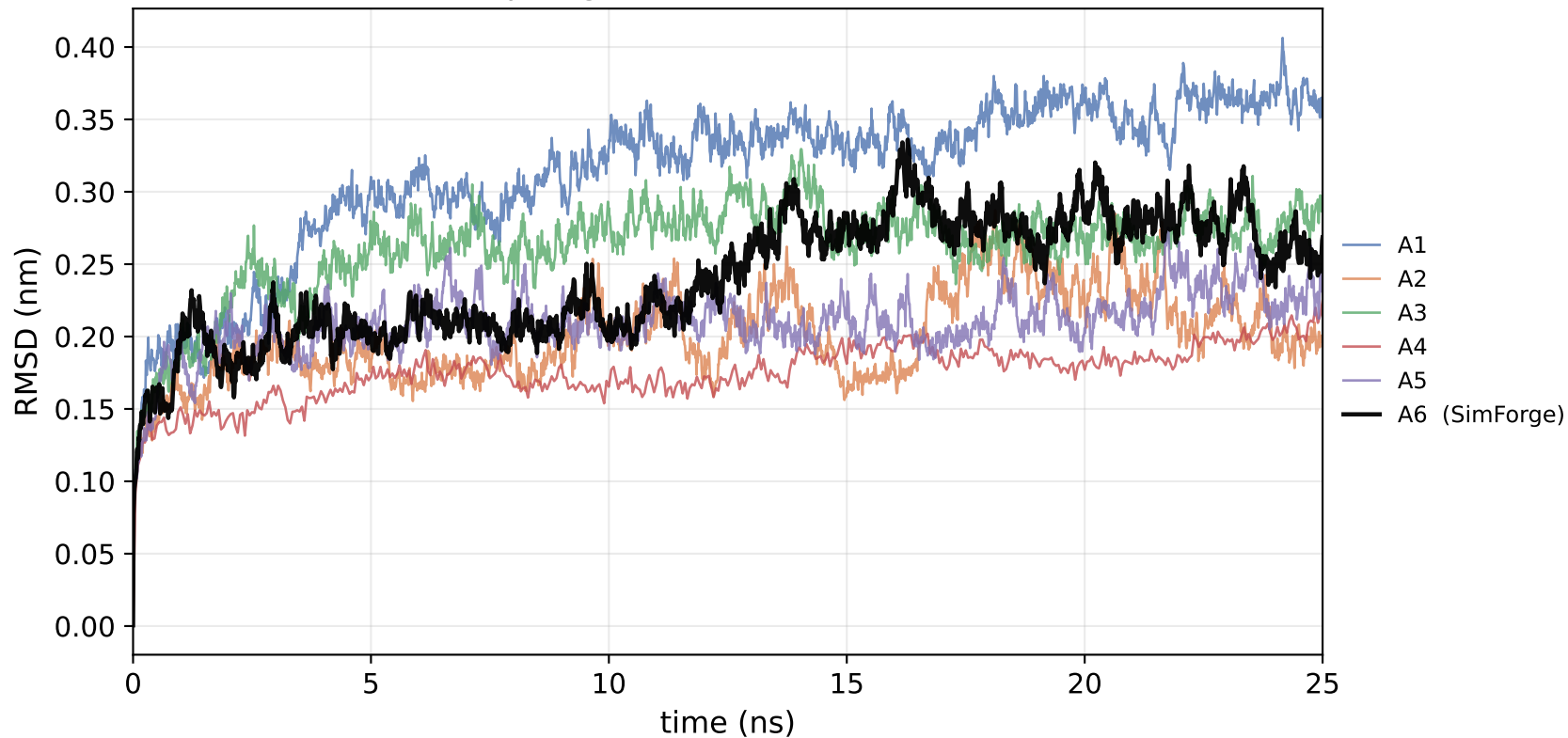
AG (alpha-glucosidase) - Protein RMSD
