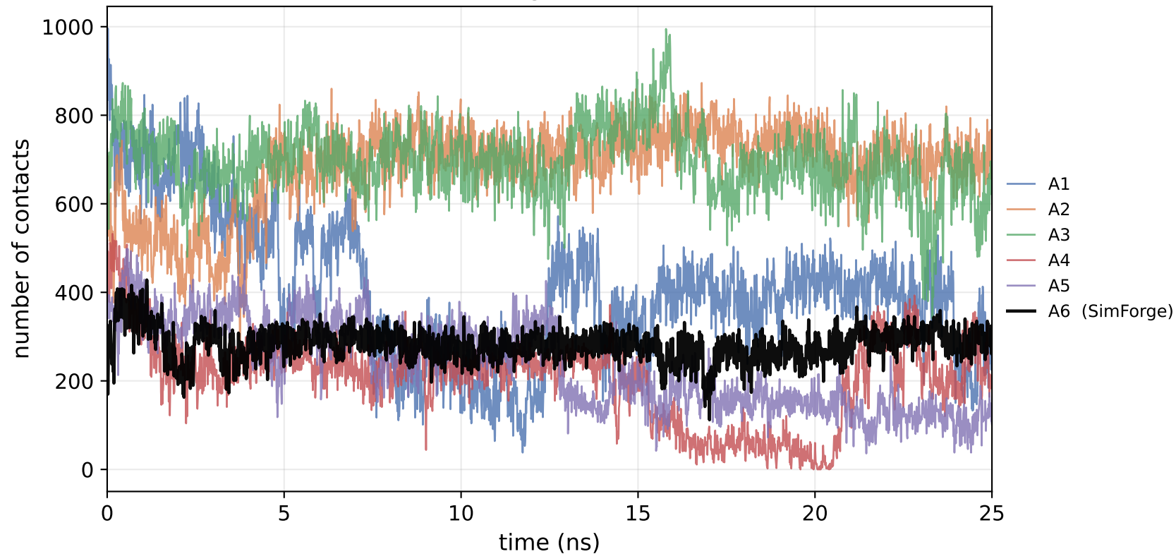
HMG (HMG-CoA reductase) - Ligand-active-site contacts (<0.6 nm)
