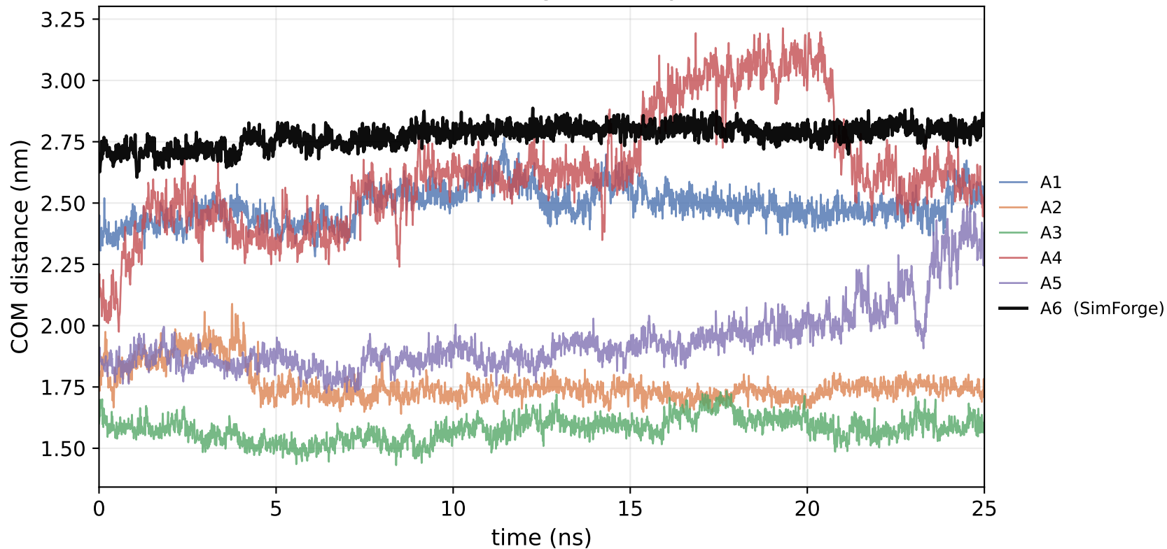
HMG (HMG-CoA reductase) - Ligand-catalytic-site COM distance
