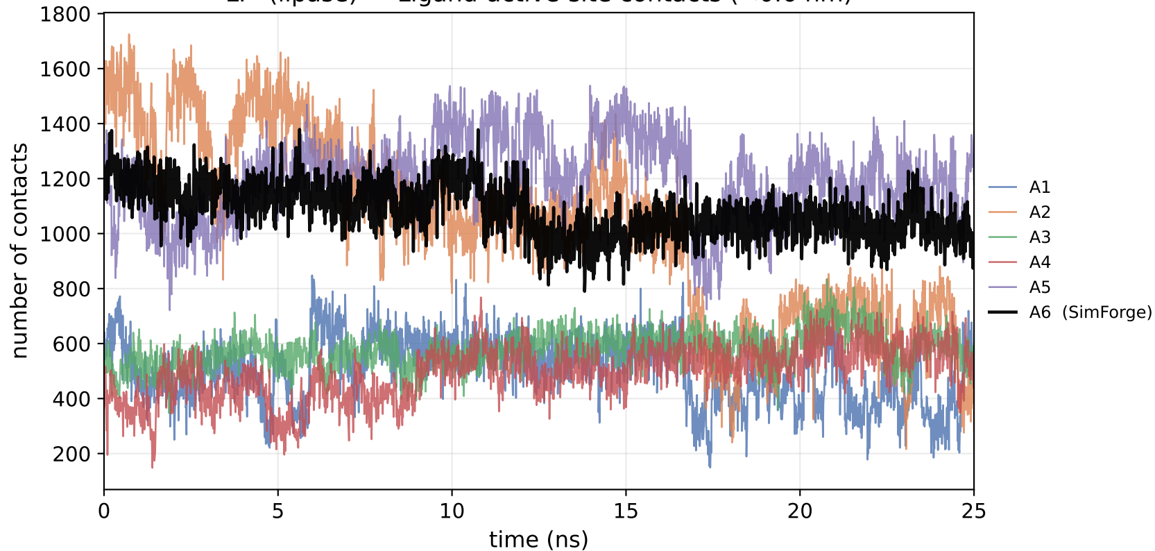
LP (lipase) - Ligand-active-site contacts (<0.6 nm)
