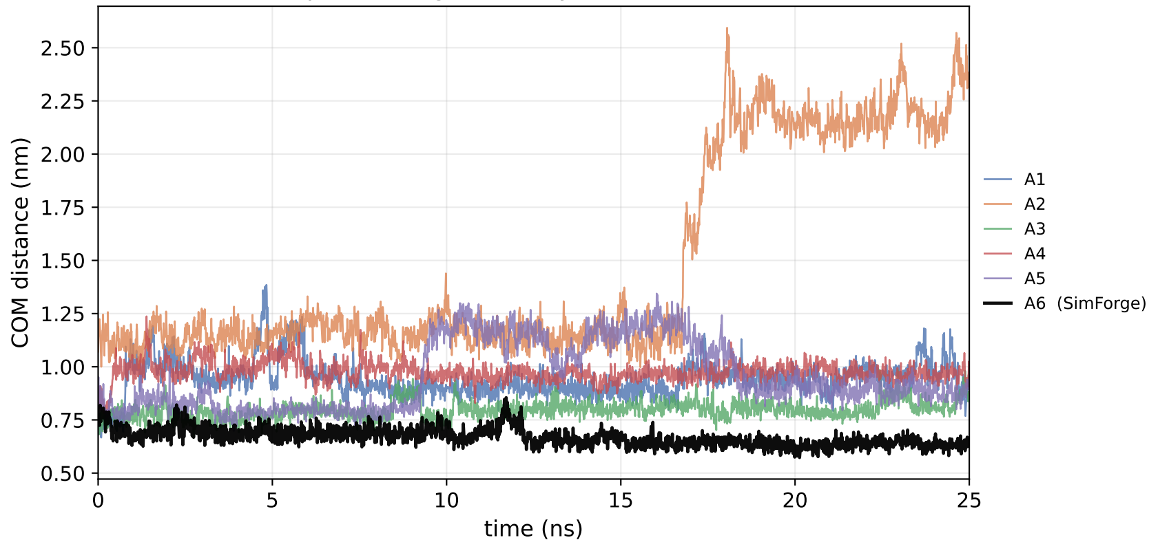
LP (lipase) - Ligand-catalytic-site COM distance
