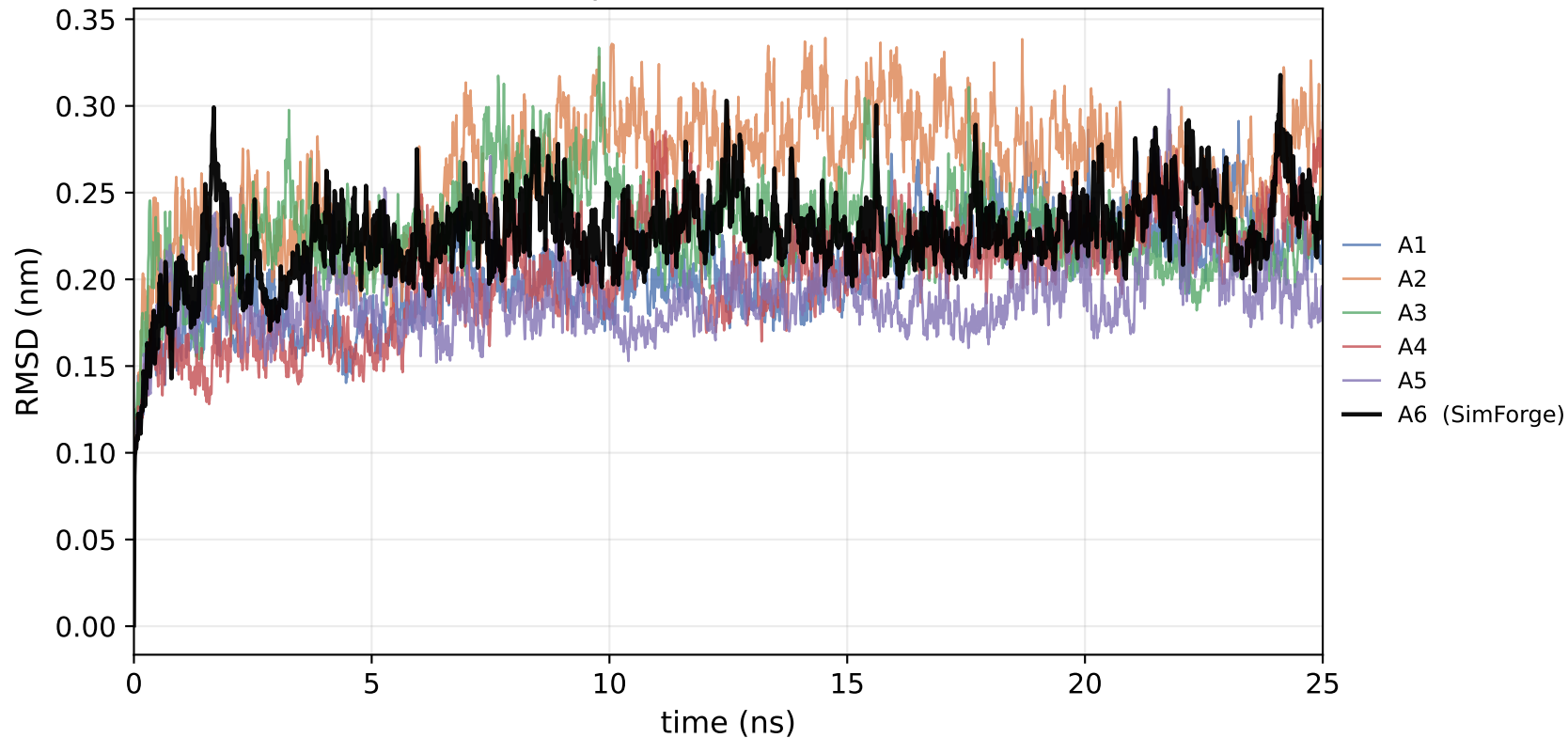
LP (lipase) - Protein RMSD
