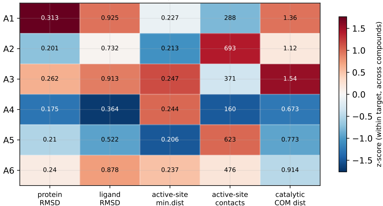
AG (alpha-glucosidase) - short-study descriptor profile (cell text = raw mean; colour = per-column z-score across A1-A6)
