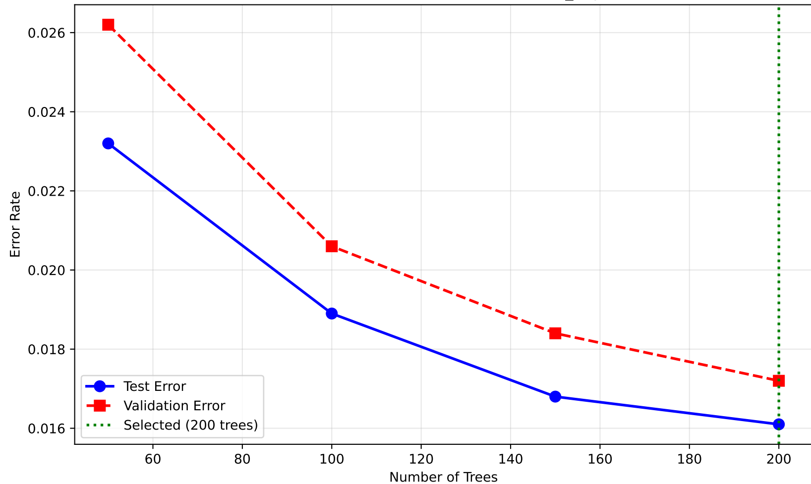
XGBoost on MNIST-LeNet5 Features (max_depth=8)
