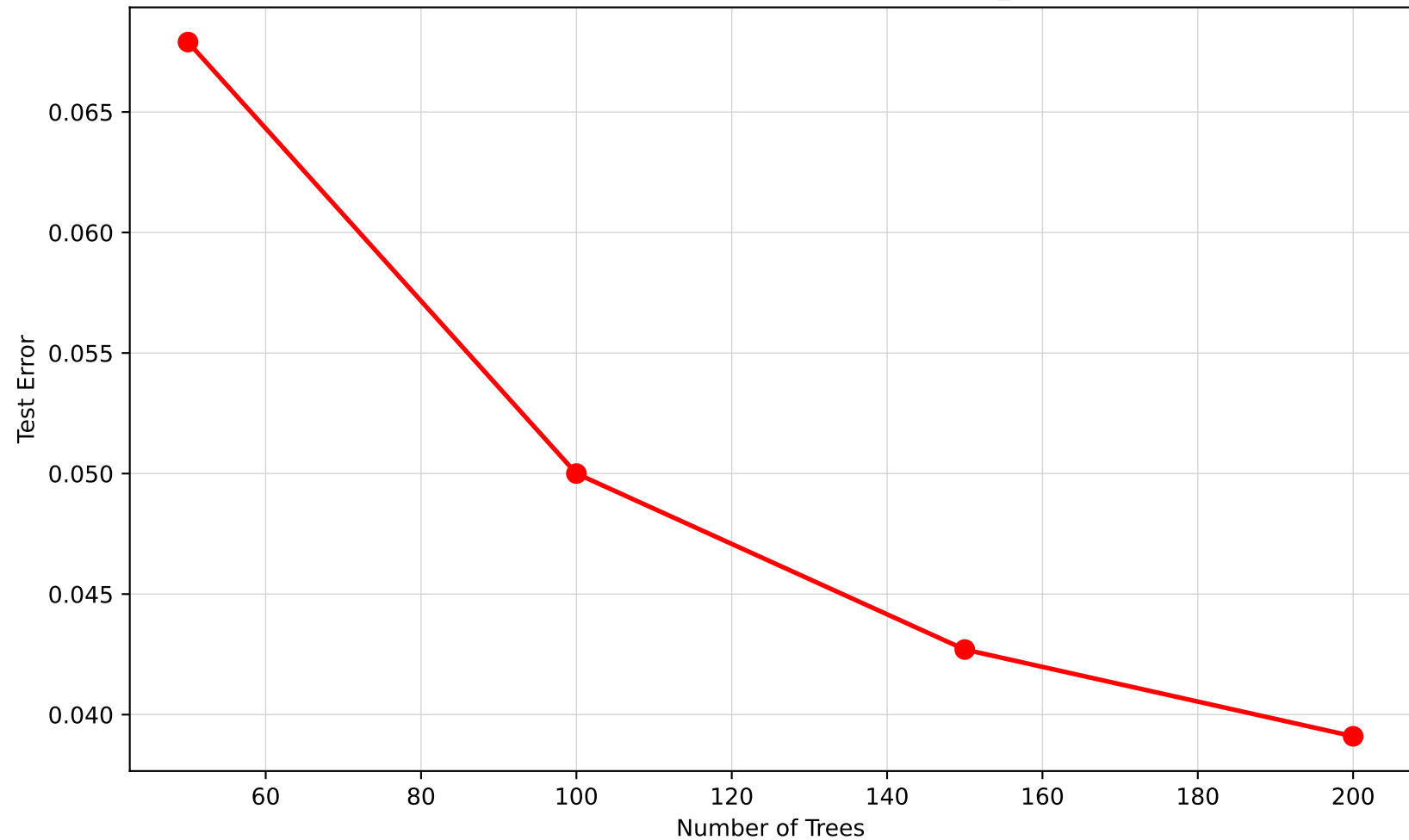
XGBoost on MNIST Pixel PCA Features (max_depth=6)
