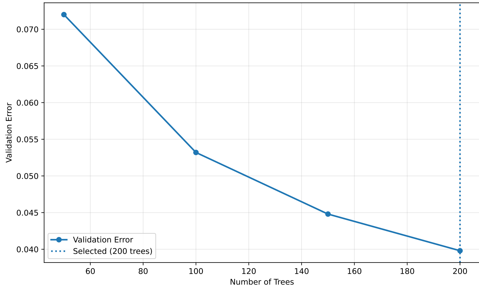
XGBoost on MNIST Pixel PCA Features
