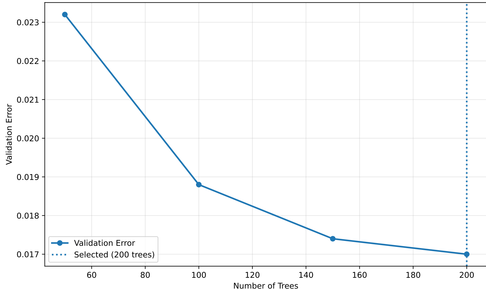
XGBoost on MNIST LeNet5 Features
