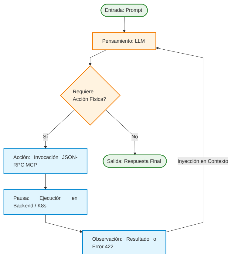
Figura 12: Diagrama de flujo del bucle cognitivo ReAct ( Reasoning and Acting ).
