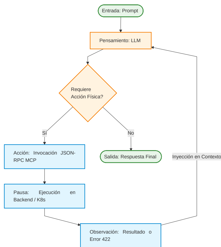
Figura 11: Diagrama de flujo del bucle cognitivo ReAct (Reasoning and Acting).
