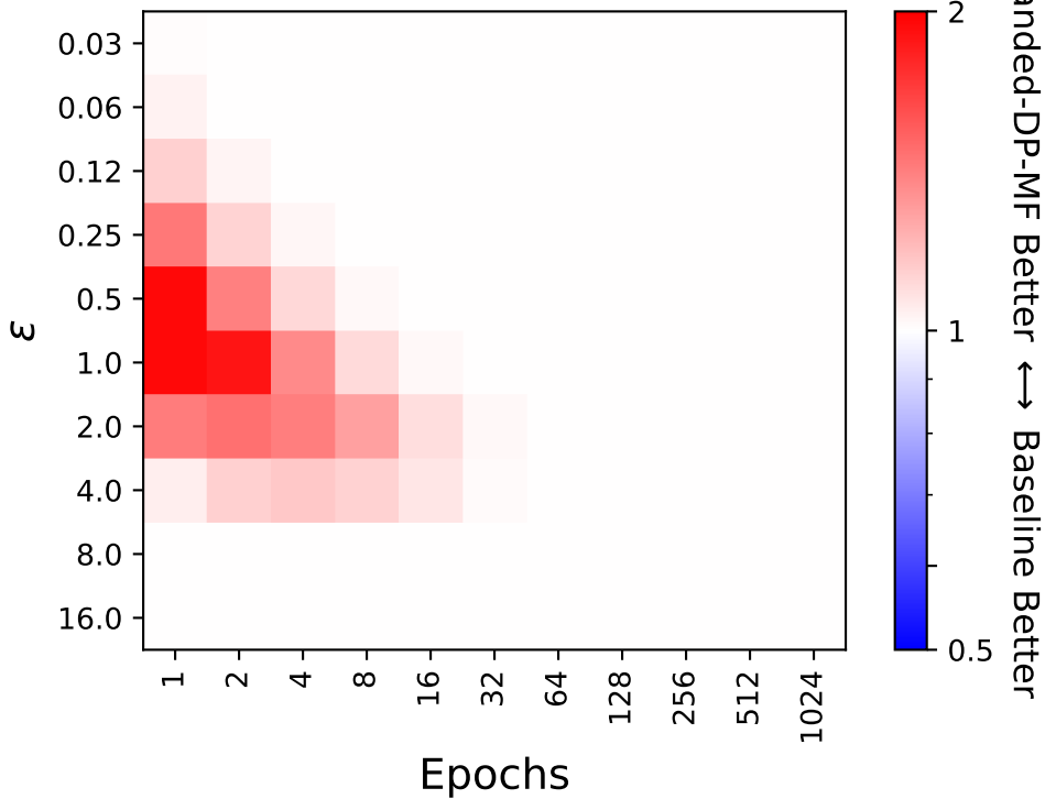
RMSE Ratio, n = 1024
