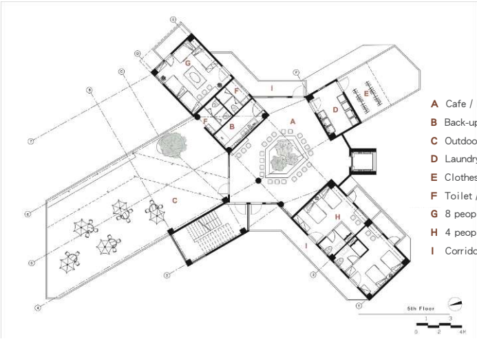
Room plan
