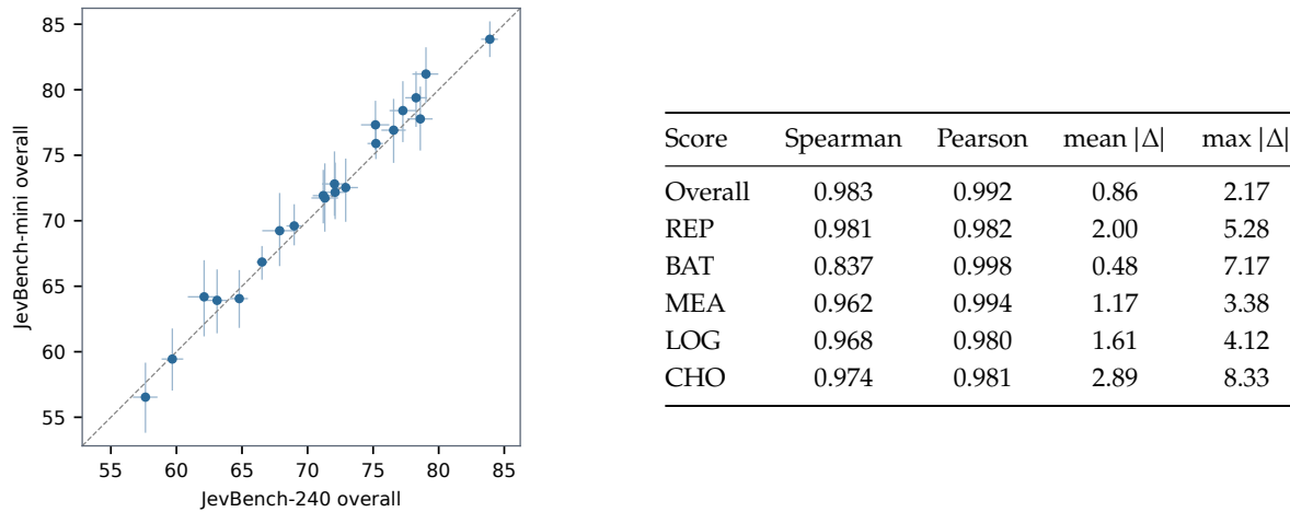
Figure 3 | Overall coherence of the 21 models run on both suites, with 95% intervals (left), and agreement of the overall and dimension scores (right; \Delta : JevBench-mini minus JevBench-240, in points).
