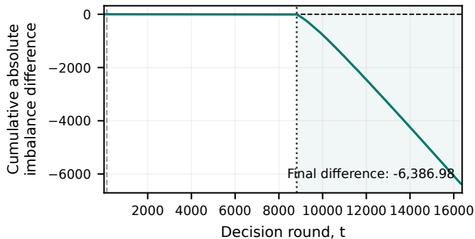
(c) One-switch - Fast only
