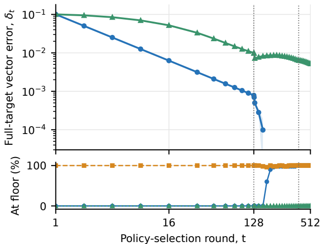
(a) Primary-run prefixes (50 paths)
