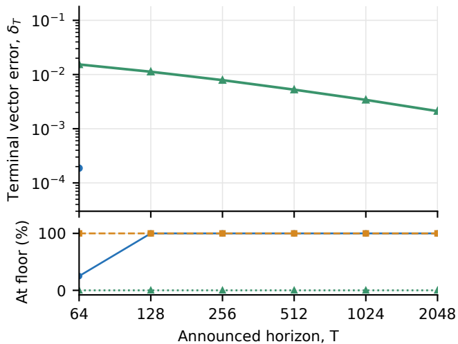
(b) Separate horizons (20 paths each)
