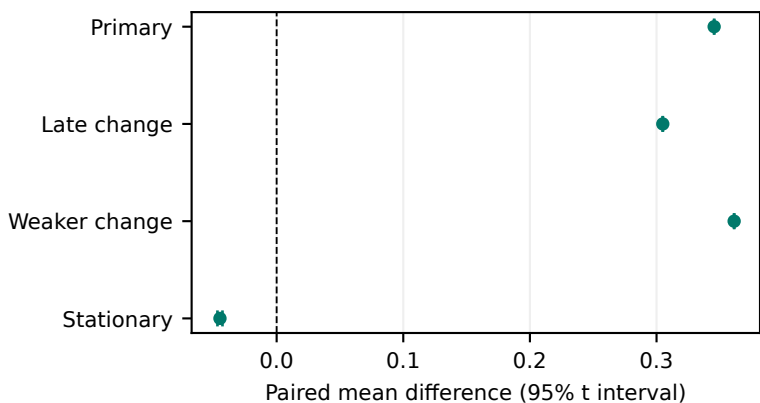
(c) Terminal distance: one-switch - block safe
