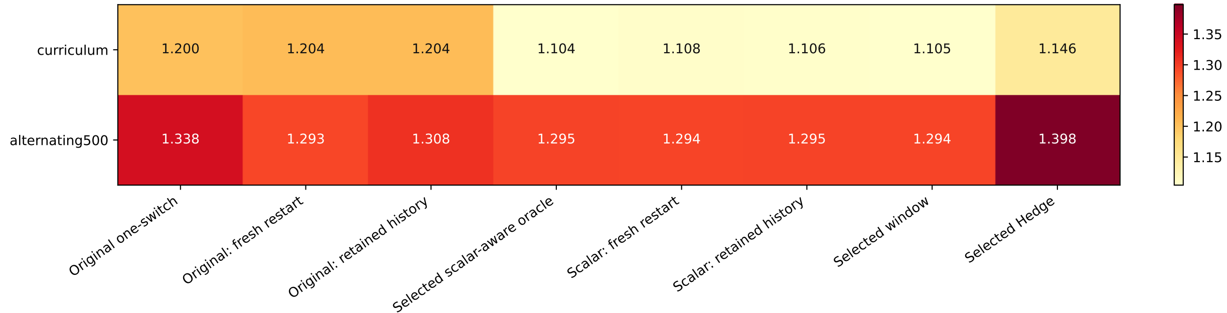
Exploratory block study: 3000 meta-rounds, blocks of 1000 Mean native loss per simulator step; lower is better
