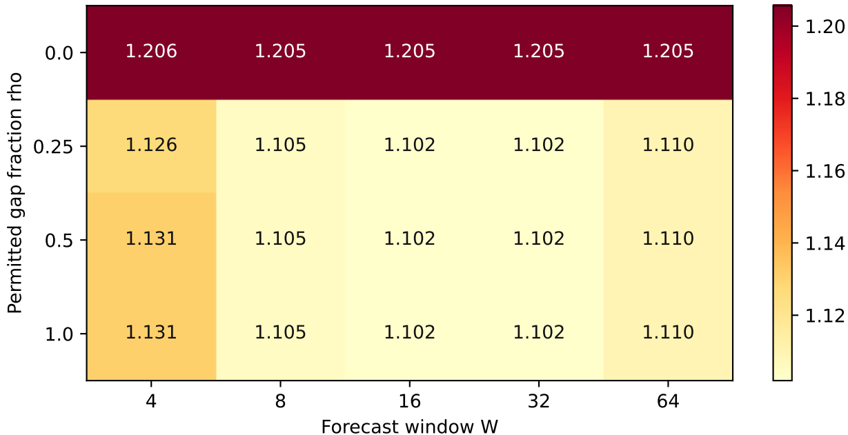
Validation grid: scalar-aware saddle oracle Selection data; no test inference
