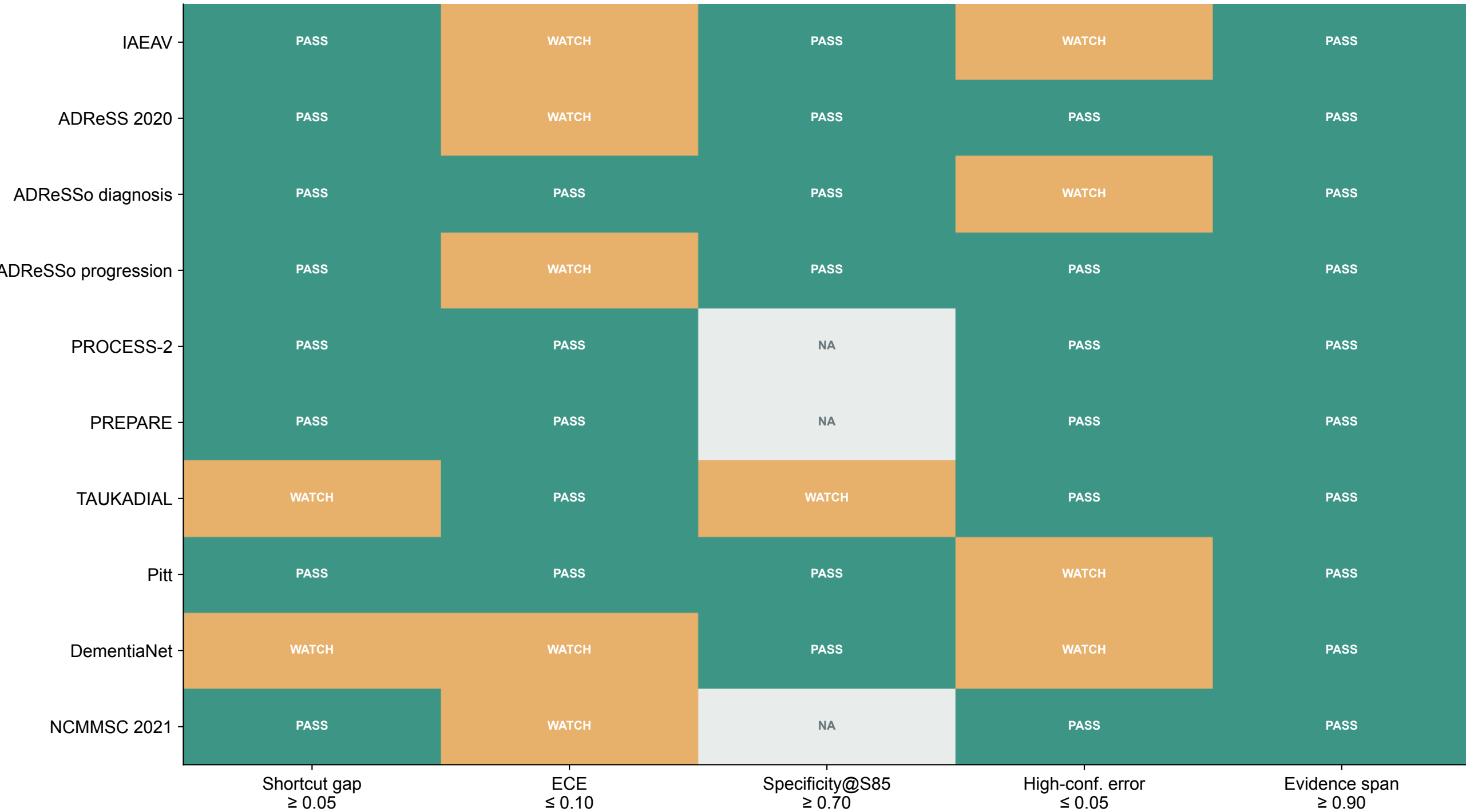
Failure-mode audit after the current framework revision
