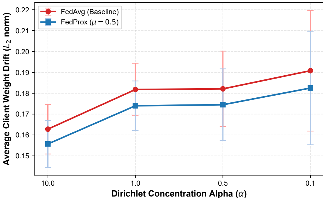
Client Drift Containment Under Heterogeneity
