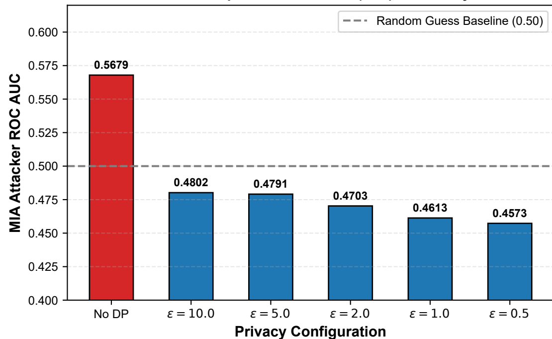
Membership Inference Attack (MIA) Sensitivity
