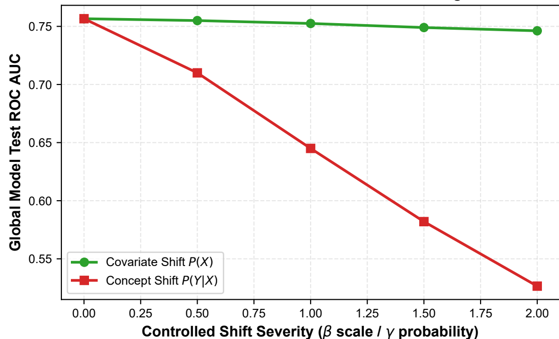
Controlled Distribution-Shift Stress Testing
