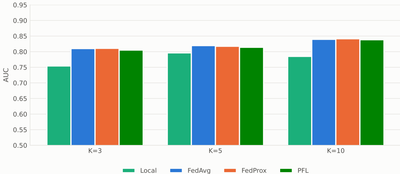
Mean per-client test AUC vs number of clients ( \alpha = 0.5 )
