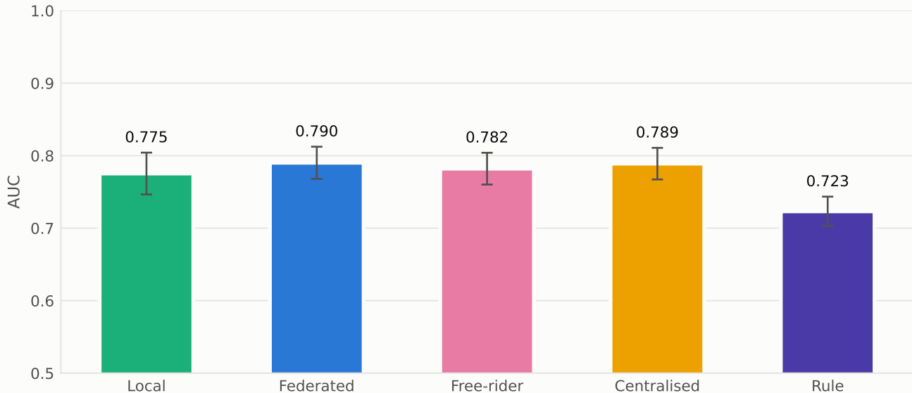
Base-paper strategies on 9 TCGA sites (mean per-site AUC, 95% CI)
