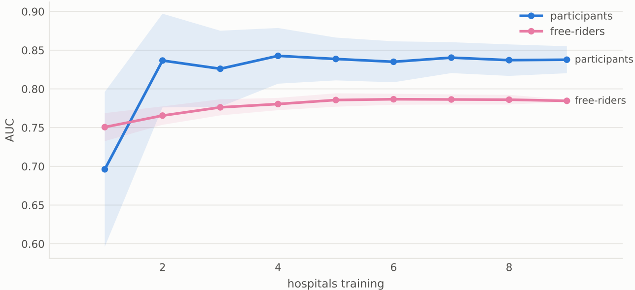
Federated AUC as hospitals join (TCGA sites)
