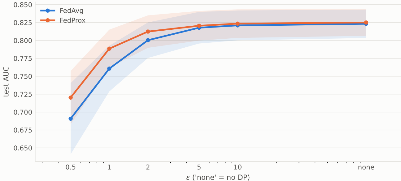
Test AUC vs privacy budget ( \alpha = 10, 20 seeds)
