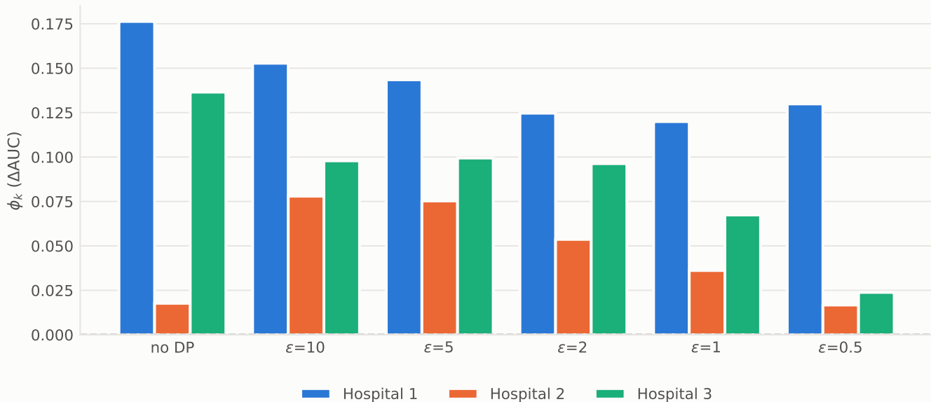
Exact Shapley values of 3 hospitals, one partition, one noise draw per \varepsilon
