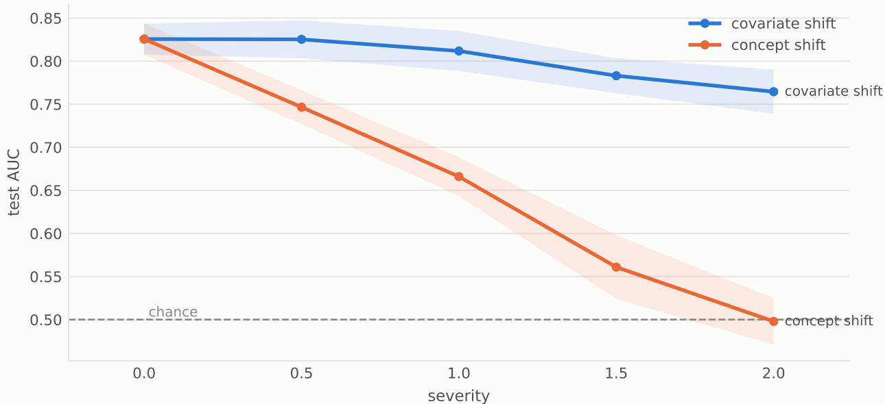
FedProx model under synthetic test-set shift
