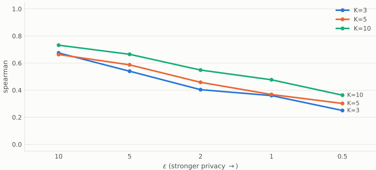
Spearman \rho with the no-DP Shapley ranking
