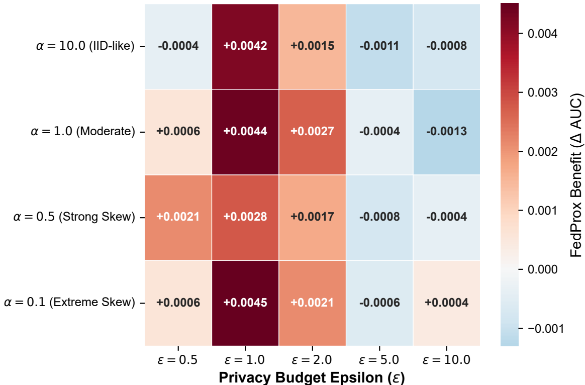
Privacy × Heterogeneity Optimization Benefit Heatmap
