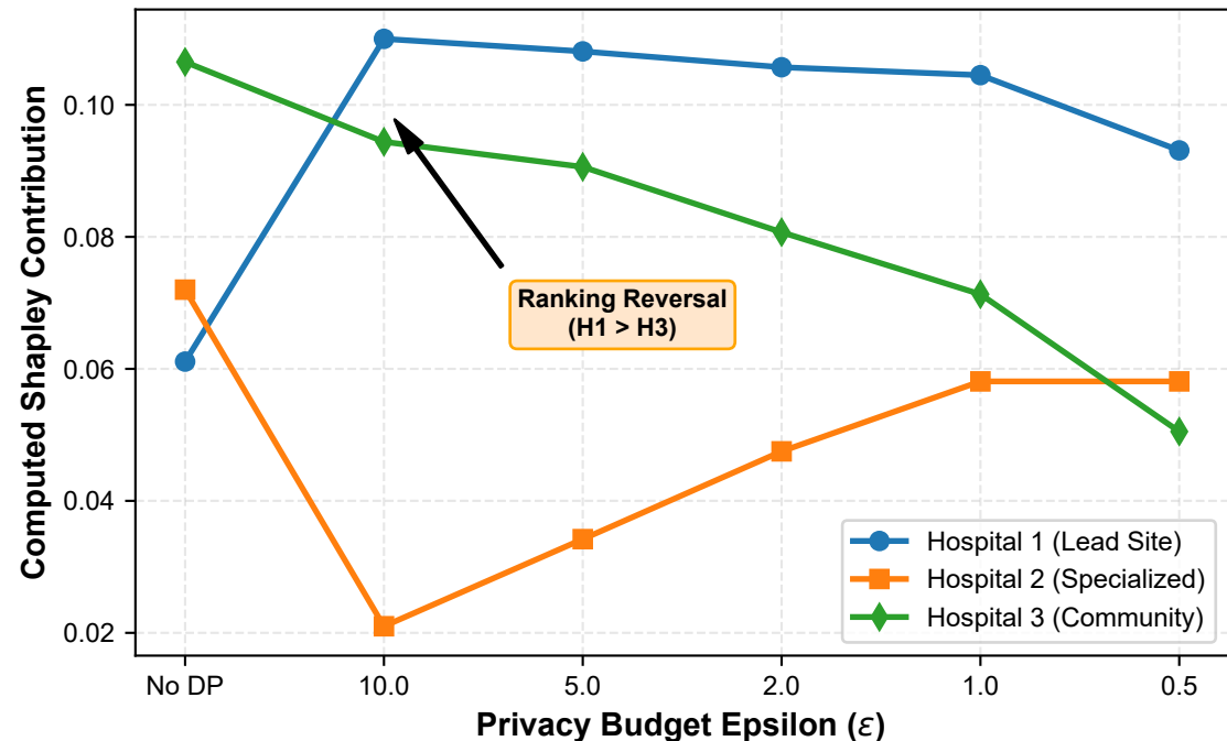
Shapley Contribution Valuation Under Privacy Noise
