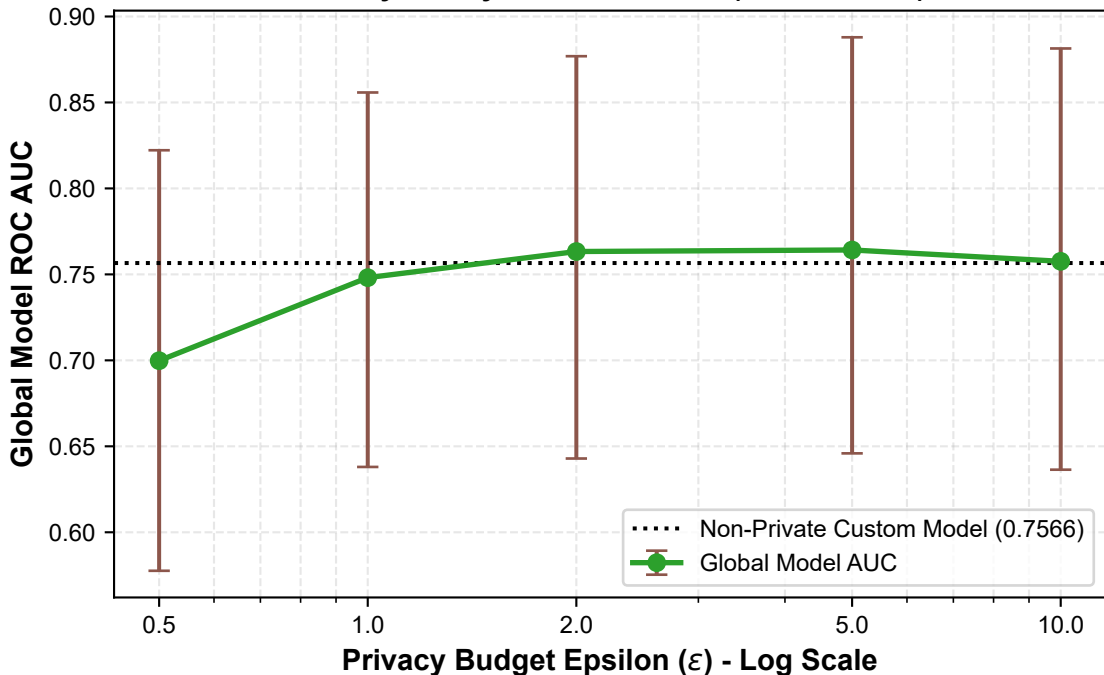
Privacy--Utility Trade-off Curve (TCGA-PRAD)
