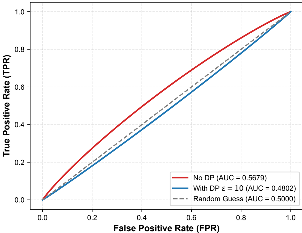
Membership Inference Attack (MIA) ROC Curves
