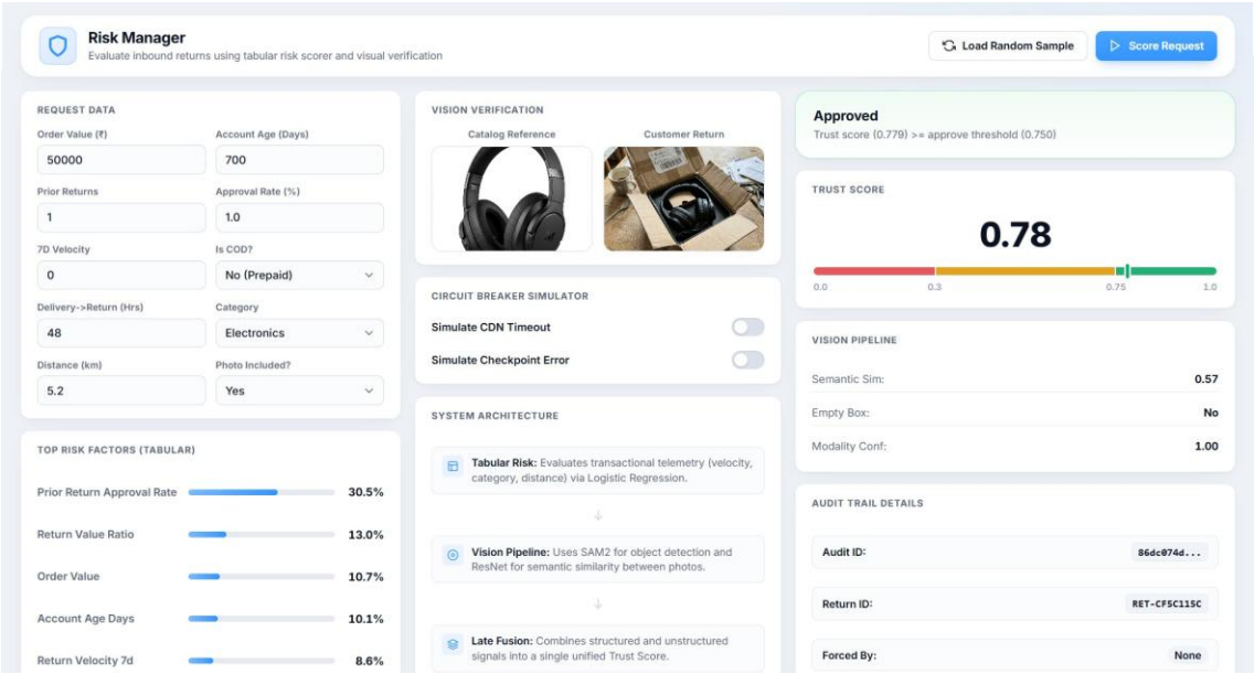
Scenario A - Auto-Approve (genuine match). A clean account (high approval-rate history, no COD) returning headphones with a return photo matching the catalog reference. Trust score 0.78, correctly routed to instant approval.
