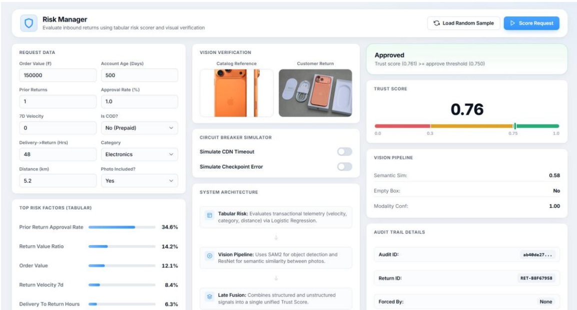
Scenario B - Auto-Approve (high-value item). A genuine iPhone return with a matching photo and low fraud indicators. Trust score 0.76, again correctly auto-approved despite the higher order value.
