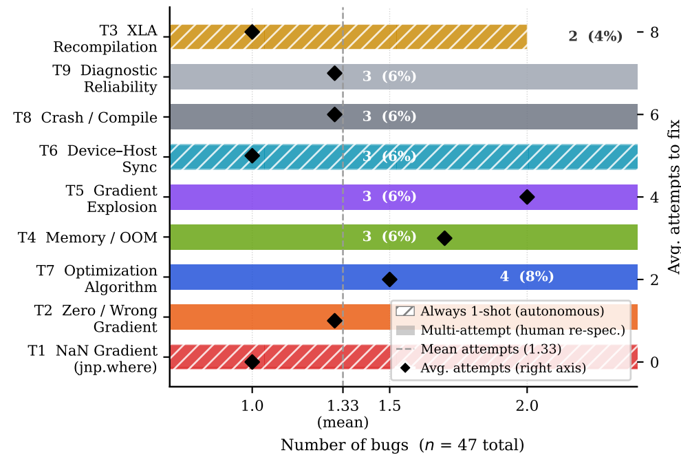
Phase 5b repair campaign: bug type distribution
