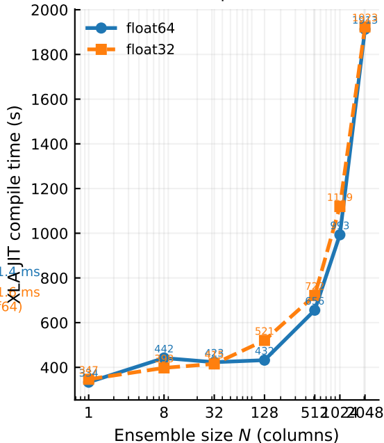
(b) XLA compile time vs N
