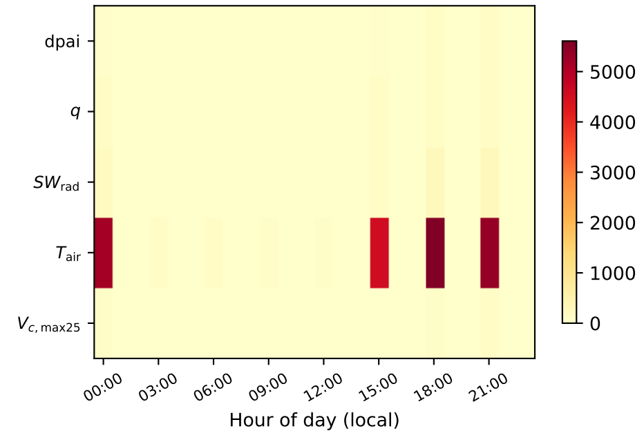
|\partial \text{LE} / \partial \theta| diurnal composite
