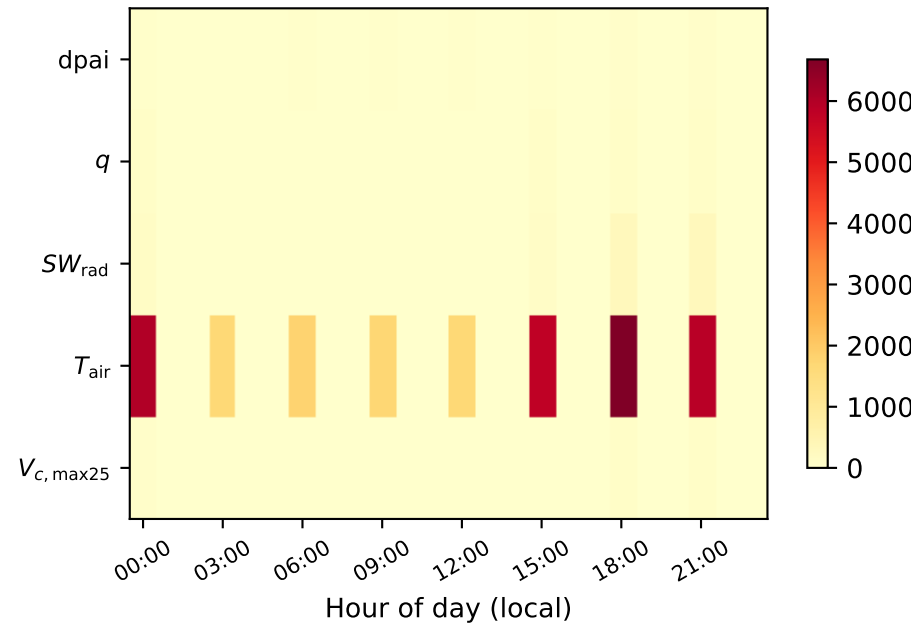
|\partial H / \partial \theta| diurnal composite
