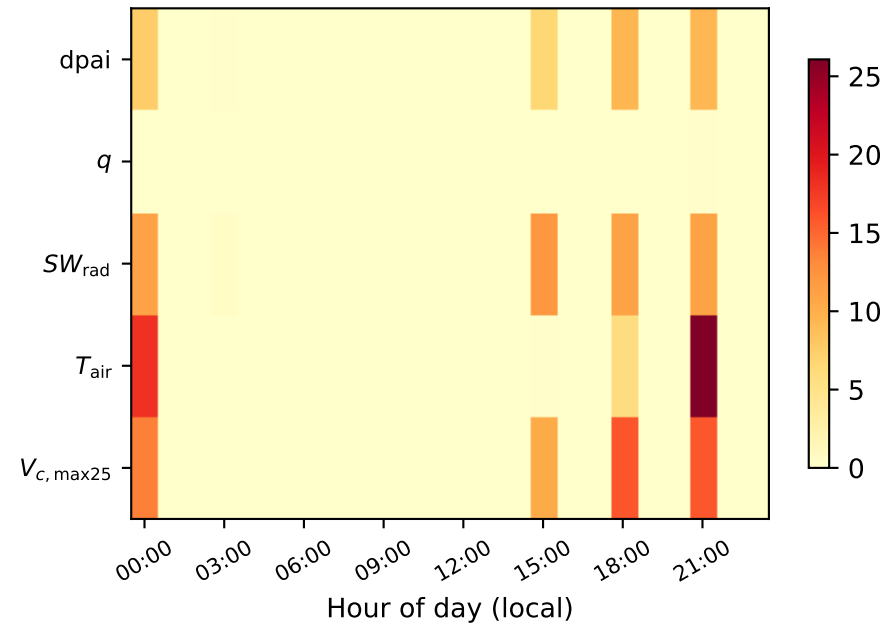
|\partial \text{GPP} / \partial \theta| diurnal composite
