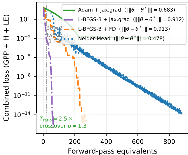
(a) Convergence — p = 10 parameters (all active)
