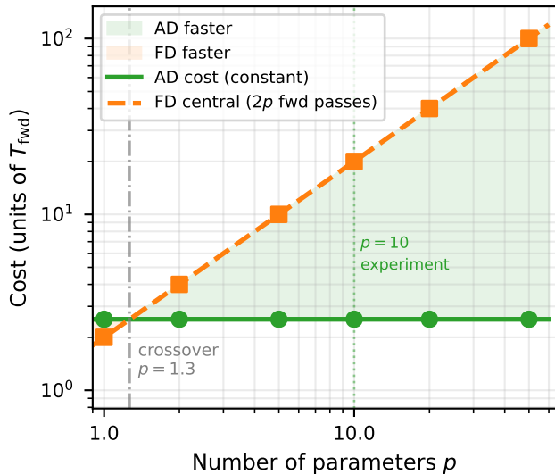
(b) Gradient cost scaling
