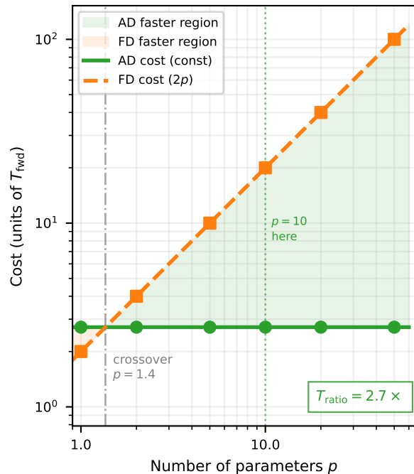
(c) Gradient cost scaling
