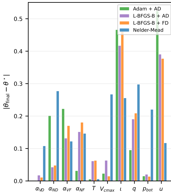
(b) Per-parameter recovery ( T = 8 steps)
