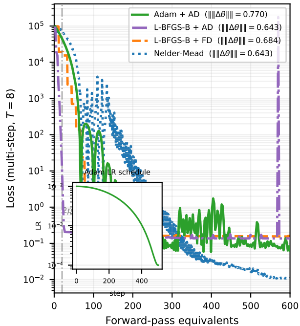
(a) Convergence — p = 10 parameters
