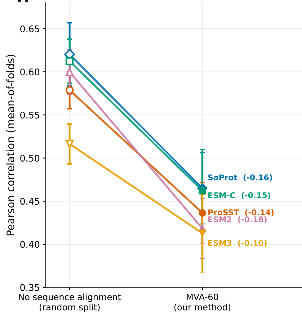
A Every encoder decays when homology leakage is removed
