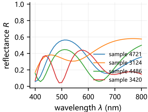
(C) TMM-generated spectra 41 points, 400-800 nm
