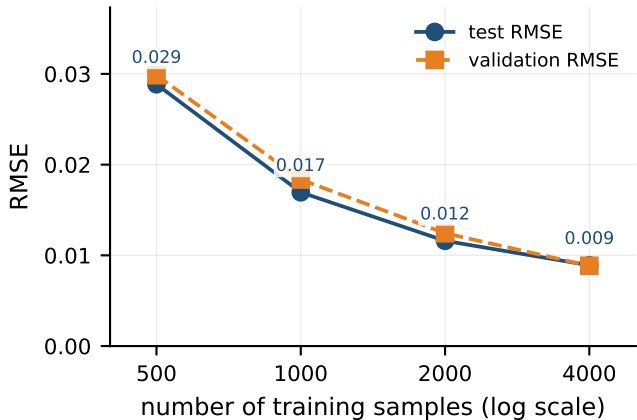
(B) error versus data volume
