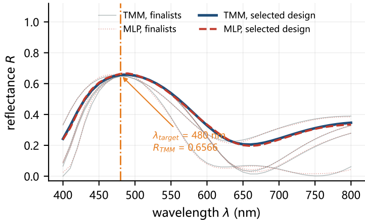
(A) selected design and the five finalists
