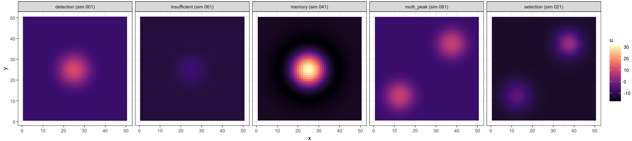
Representative 2D fields (dnfc, AbsSigmoid, Phase 1)
